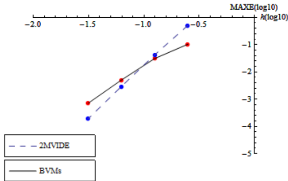
Figure 6: Graph of step sizes versus maximum errors for BVMs and 2MVIDE when solving Problem 4.
