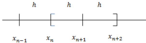
Figure 1: Two Point Multistep Block Method.
