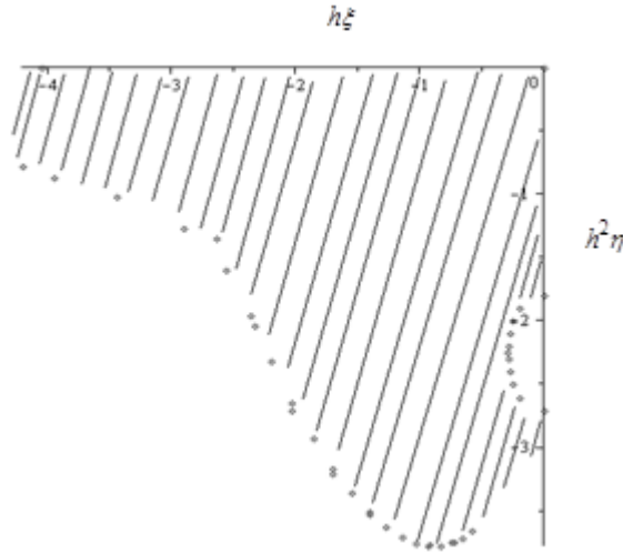
Figure 2: Stability region in the h\xi, h^2\eta plane.
