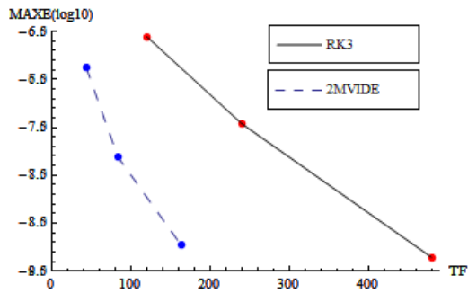
Figure 4: Graph of total functions versus maximum errors for RK3 and 2MVIDE when solving Problem 2.
