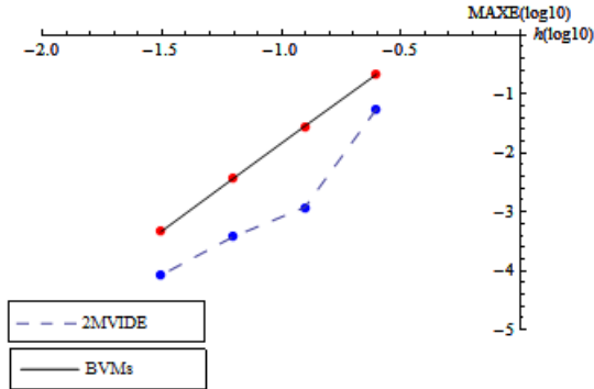
Figure 5: Graph of step sizes versus maximum errors for BVMs and 2MVIDE when solving Problem 3.
