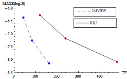
Figure 3: Graph of total functions versus maximum errors for RK3 and 2MVIDE when solving Problem 1.
